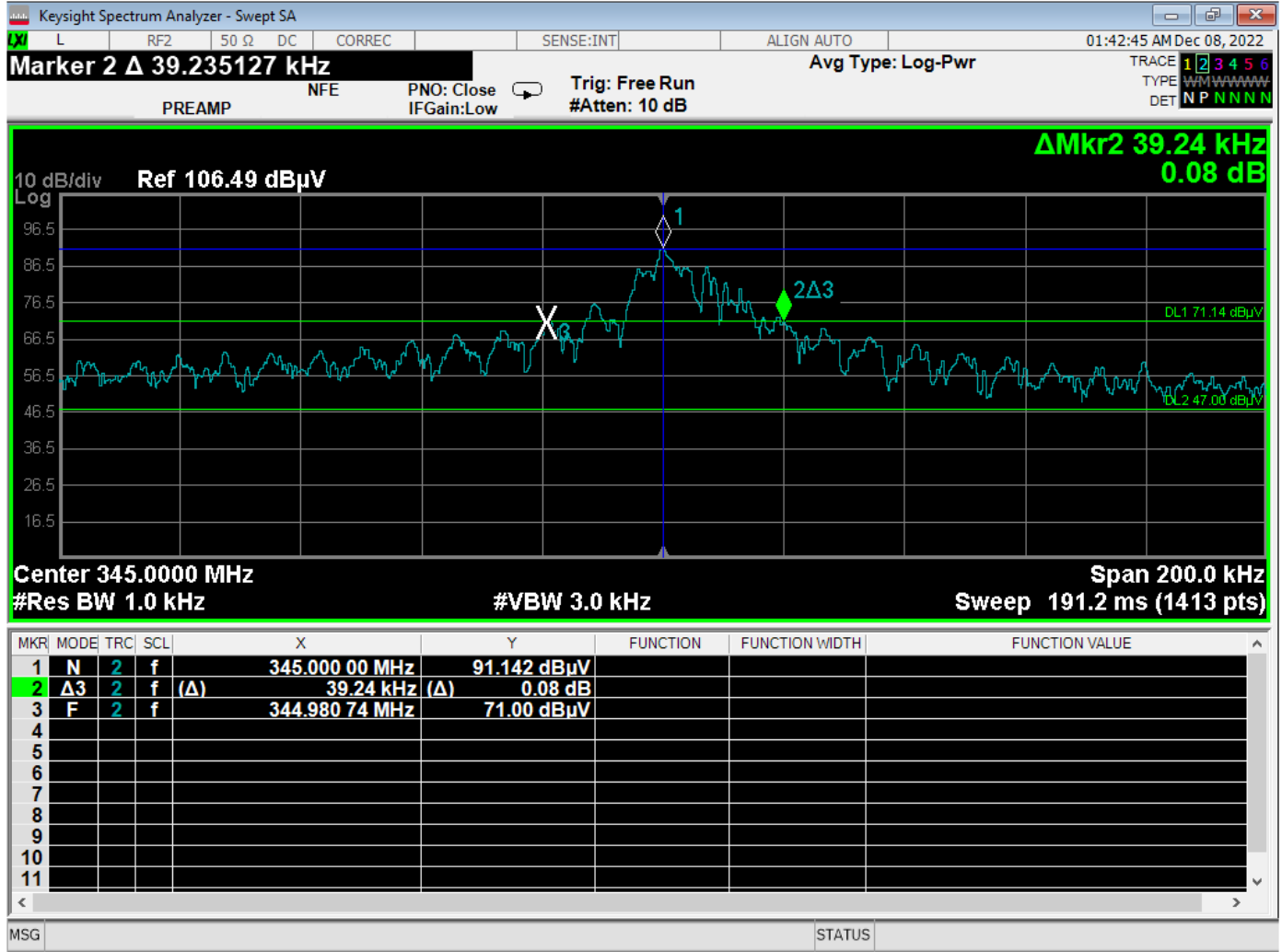
-20 dB Bandwidth Plot – No External Sensor Adapter – 1 kHz RBW
