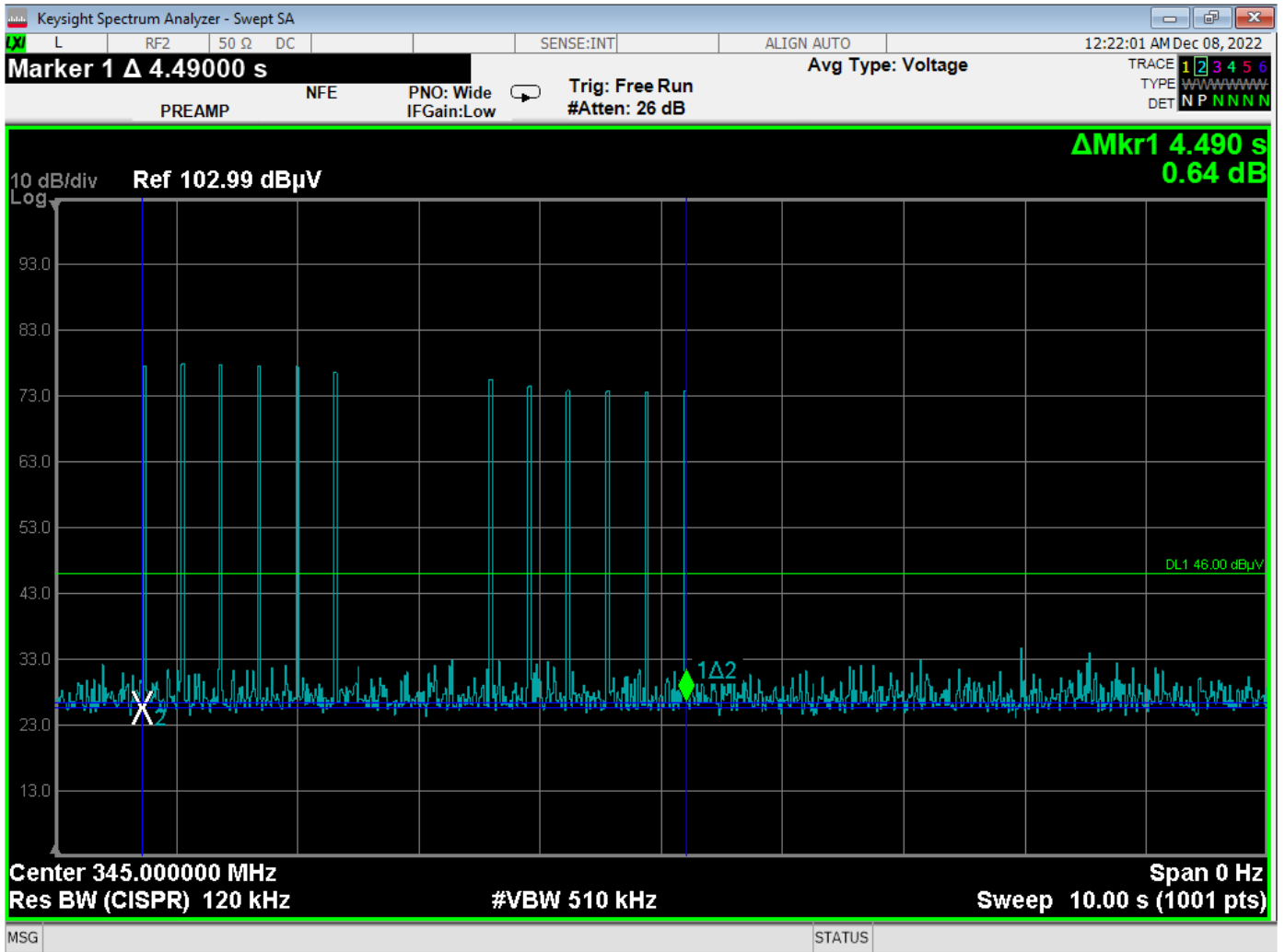
Plot Showing Actual Time of Transmission 4.49 seconds
