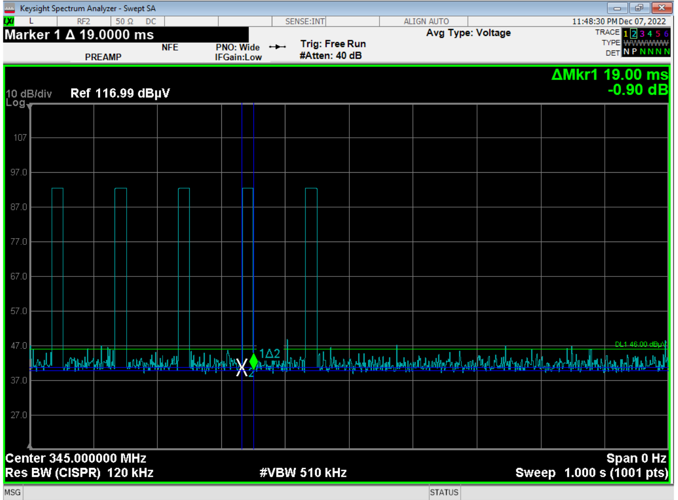
Time of One Complete Pulse Train
