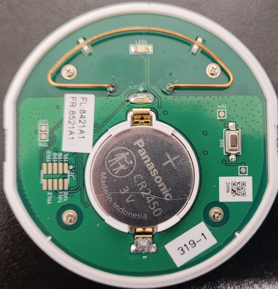
Top View of the PCB for the EUT
