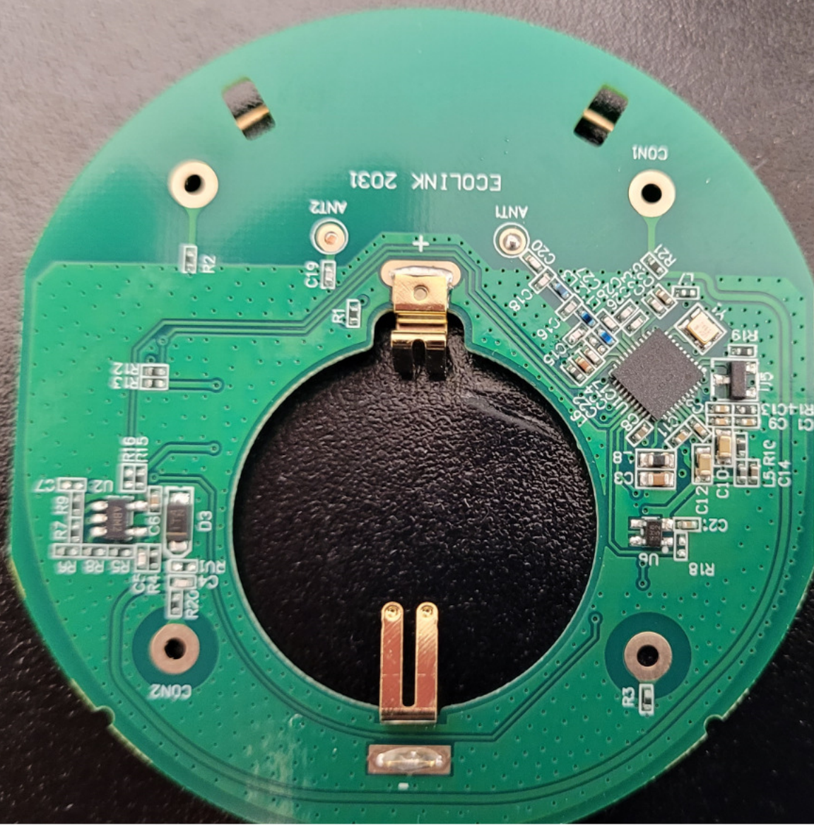
Bottom View of the PCB for the EUT
