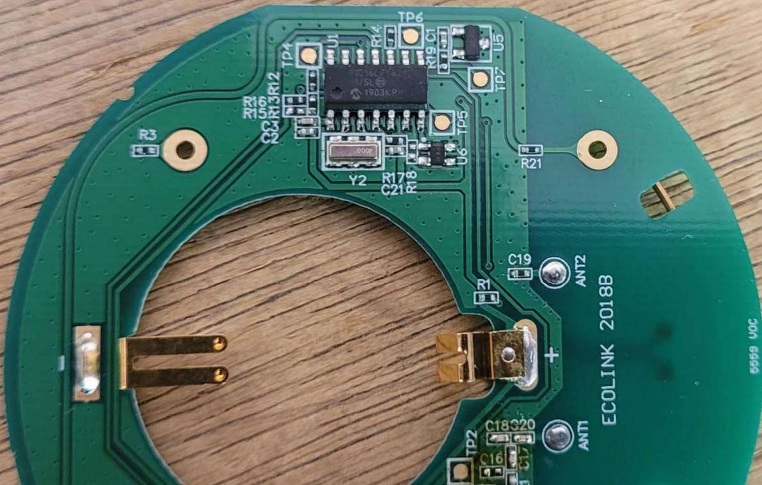
Bottom View of the PCB - Closeup #2
