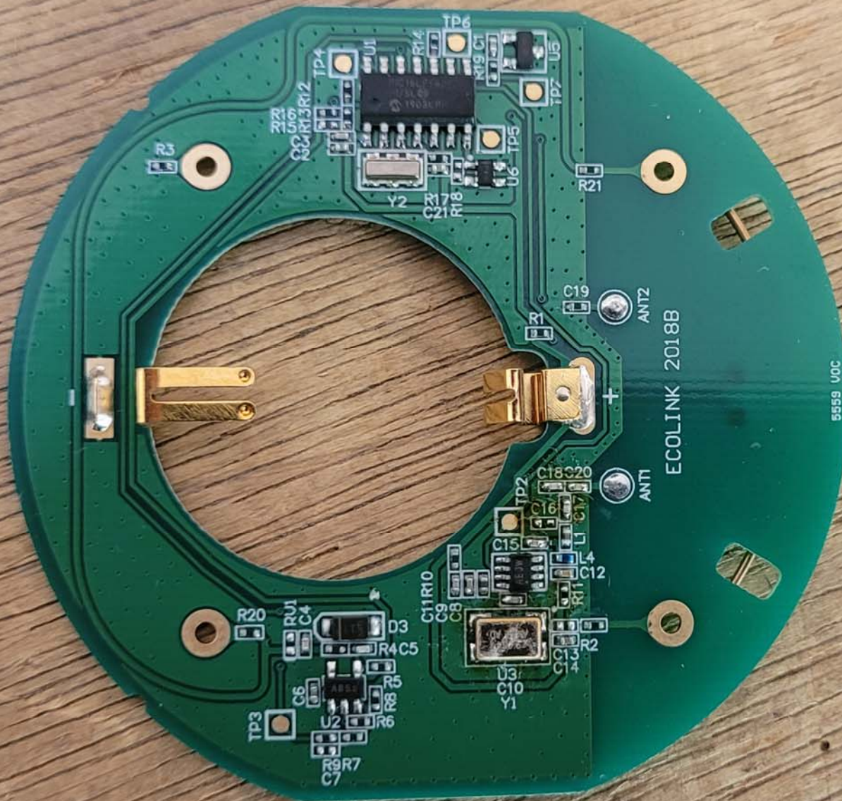
Bottom View of the PCB - Closeup #5
