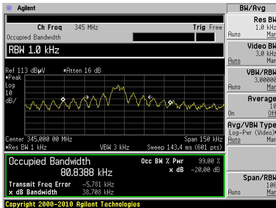
Emission Bandwidth
