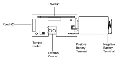
Figure 3: Circuit Board Layout
