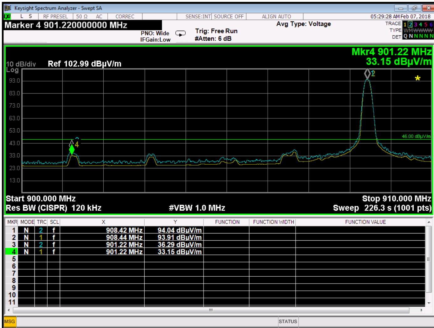
Band Edge - 908.42 MHz - Horizontal - X-Axis - Worst Case
