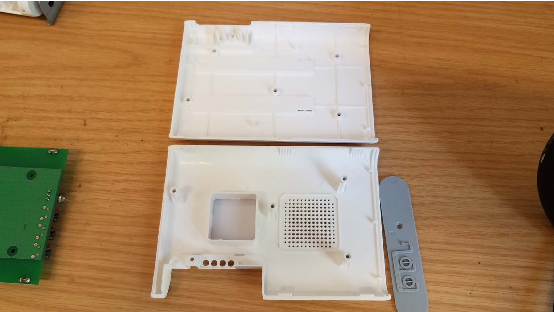
Inside View of the EUT - PCB's Removed
