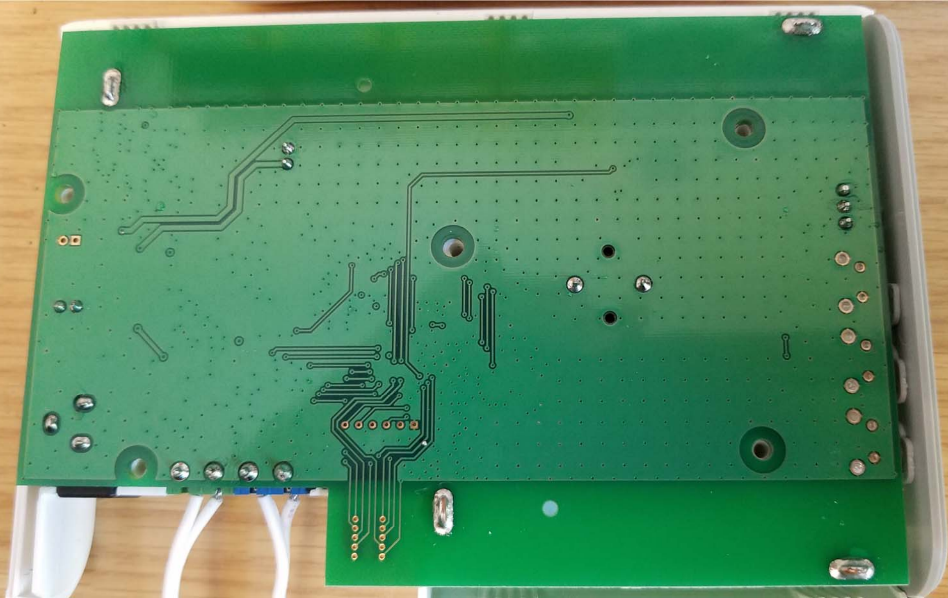
Bottom View of the PCB - View #2
