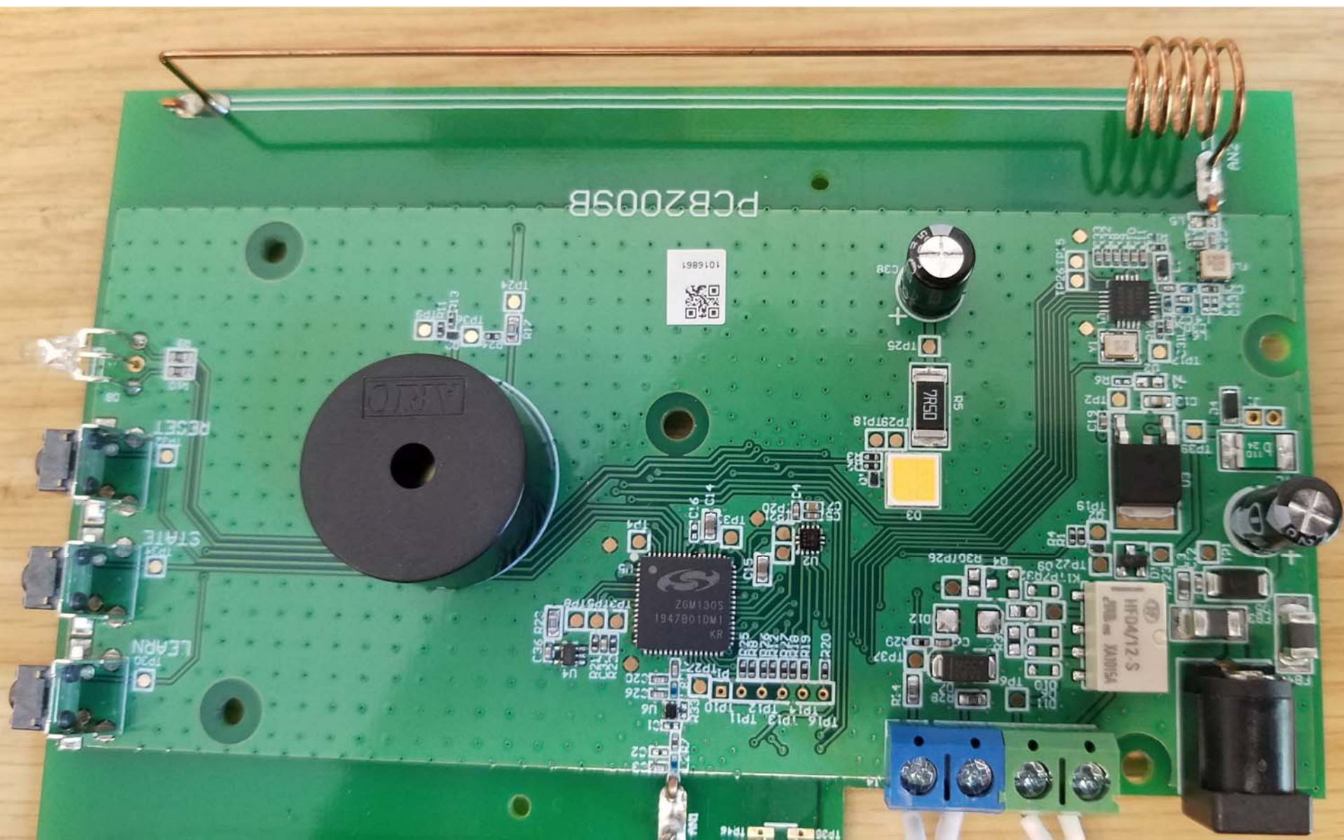
Top View of the PCB - Closeup #1
