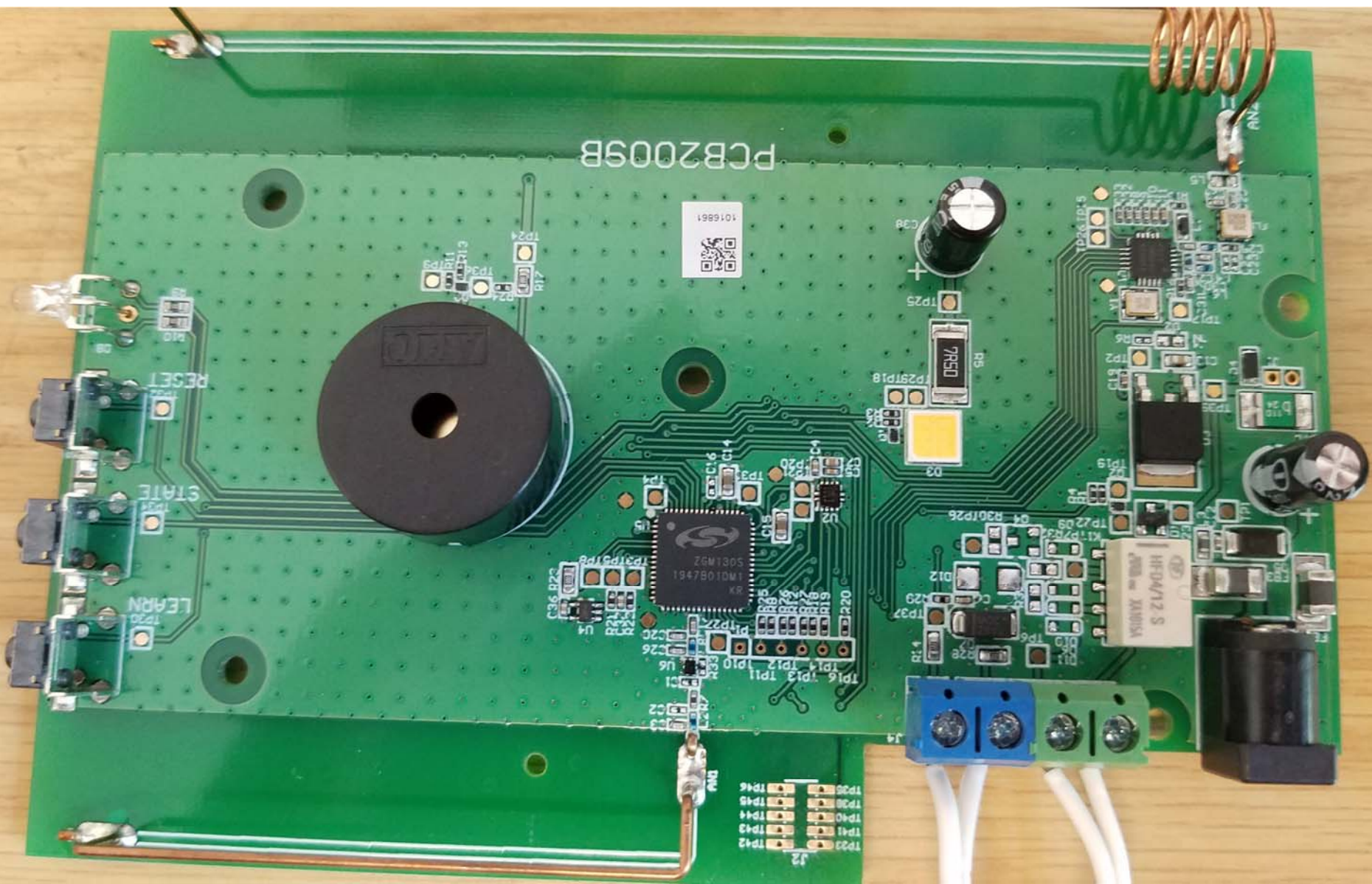
Top View of the PCB - View #2
