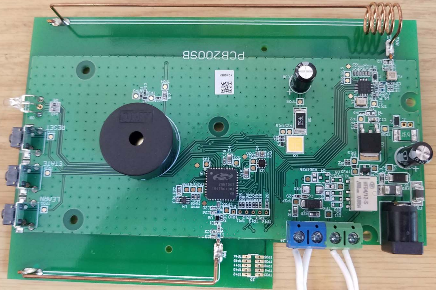
Top View of the PCB - View #1
