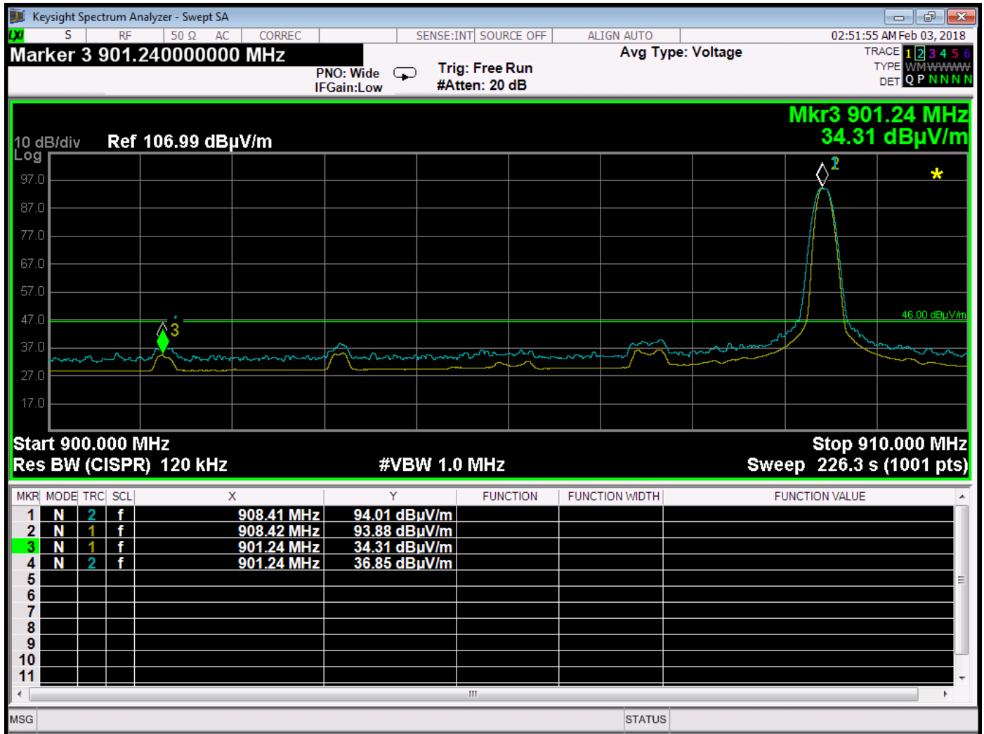
Band Edge - 908.42 MHz - Horizontal - X-Axis - Worst Case
