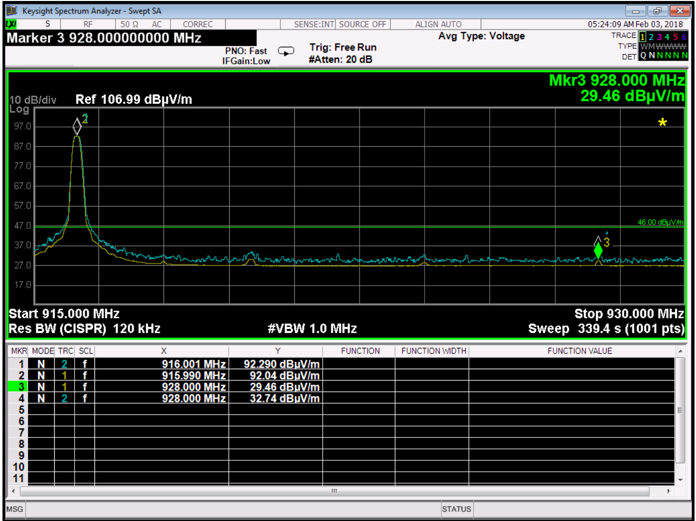
Band Edge - 916 MHz - Vertical - Y-Axis - Worst Case
