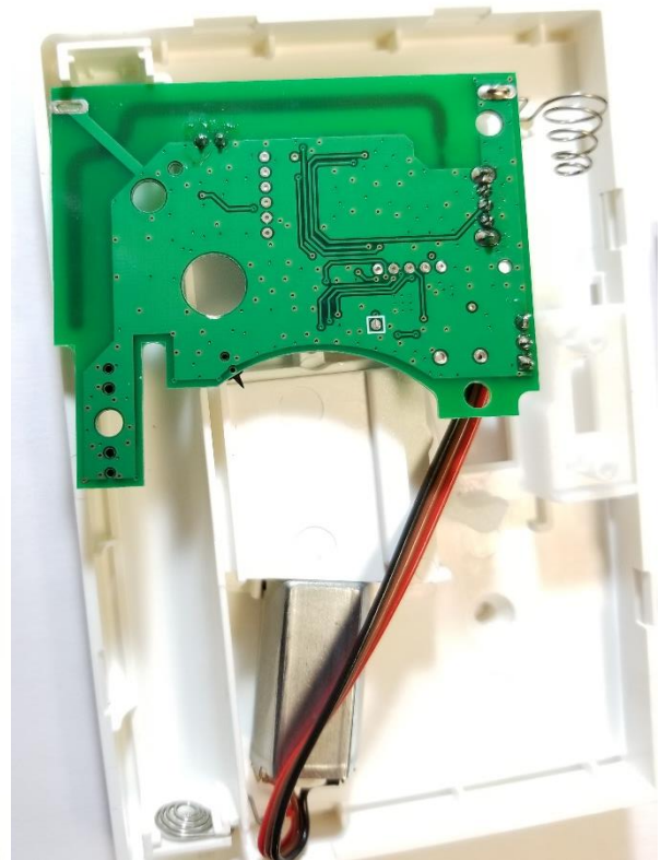
Back PCBA
