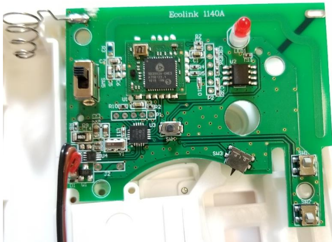
Front PCBA
