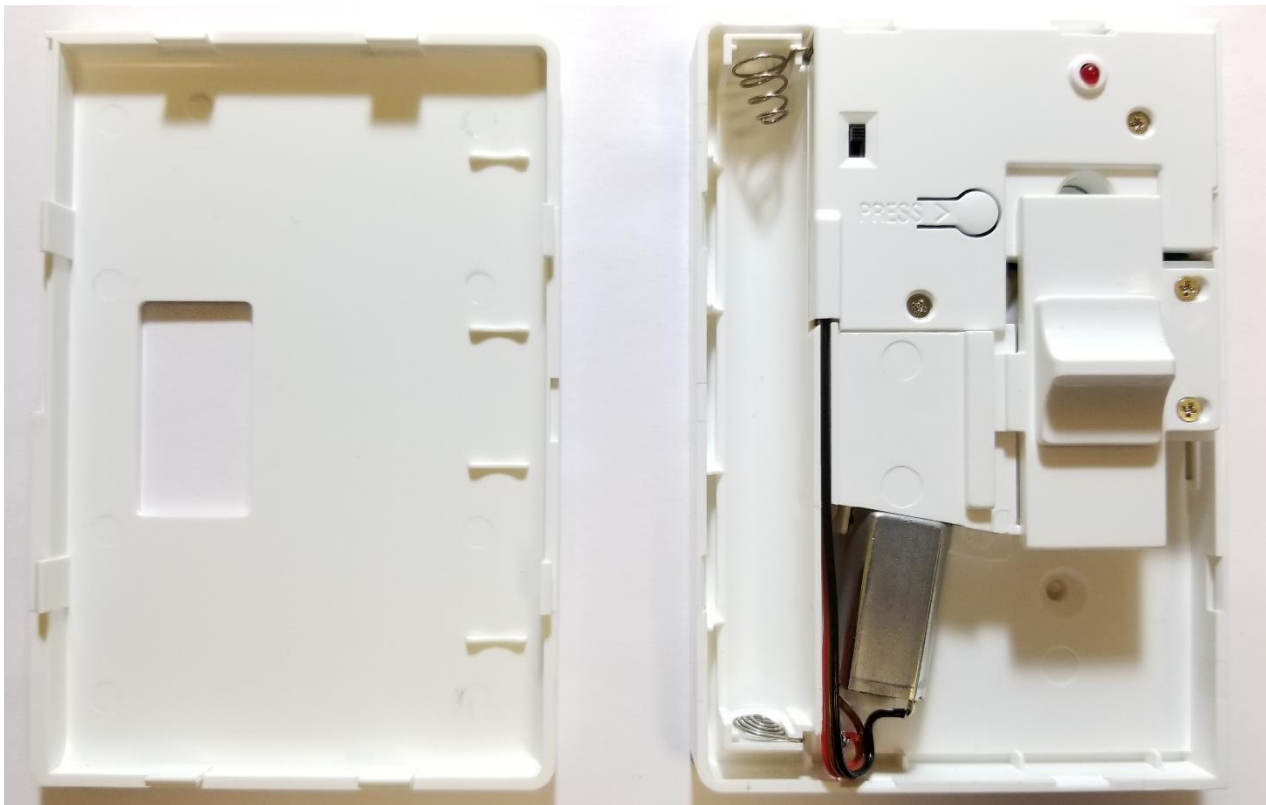
Front plate – back
