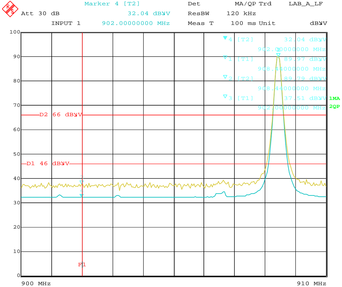
Band Edge - 908.42 MHz - Vertical - Y-Axis - Worst Case
