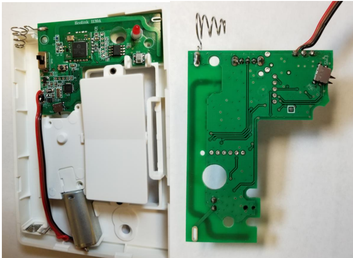
Front PCBA
