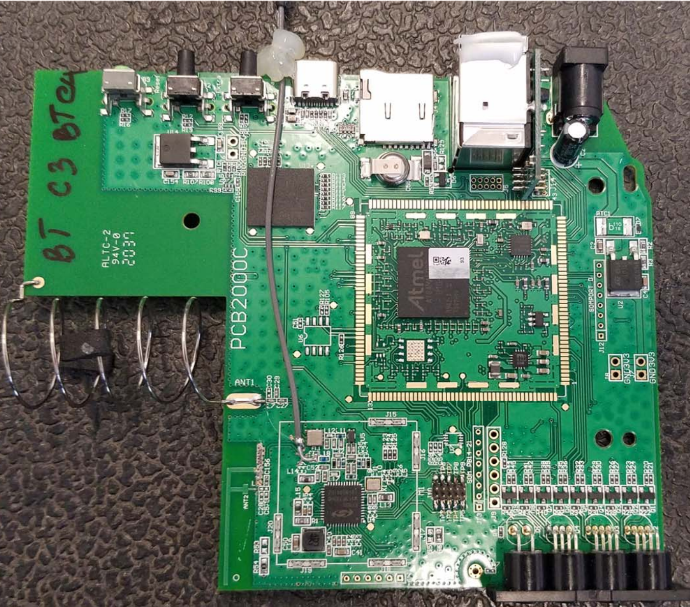
Top View of the PCB with Shield Removed - View #1
