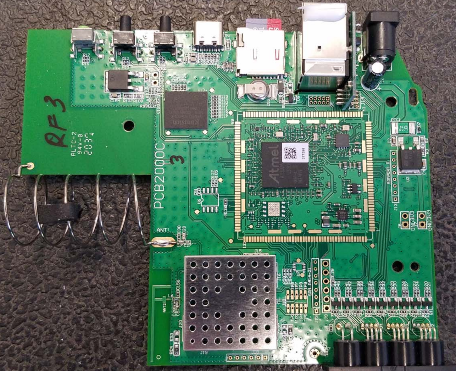
Top View of the PCB with Shield - View #1
