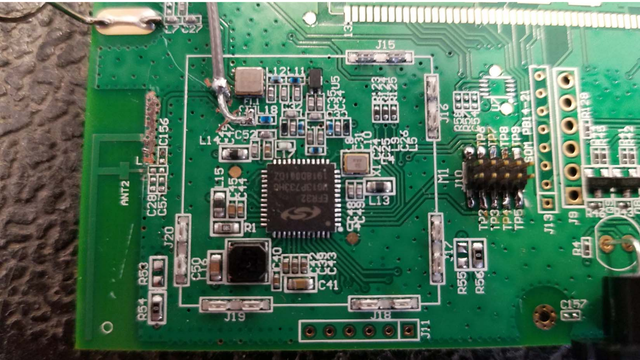
Top View of the PCB - Closeup of Area with Shield Removed
