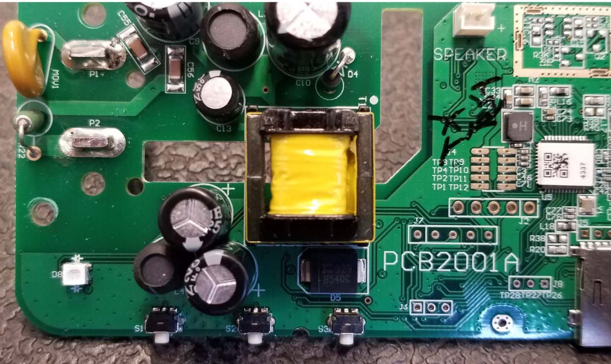
Top View of the PCB - View #3
