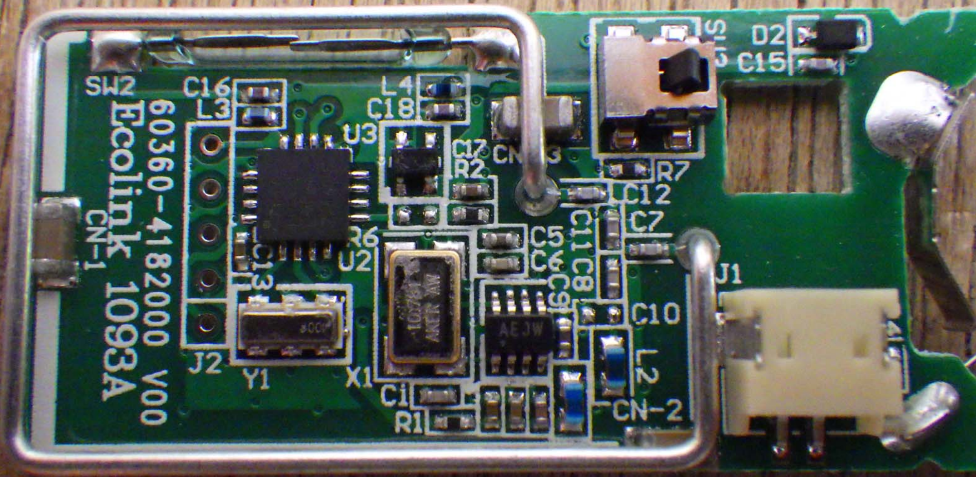
Top View of the PCB - NO Sticker - View #2
