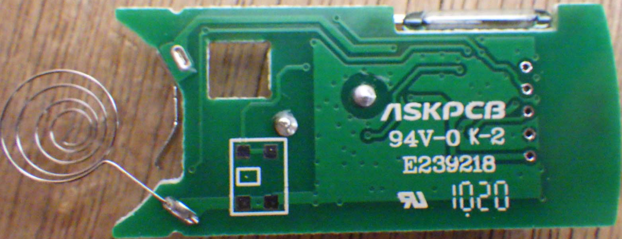
Bottom View of the PCB - View #1
