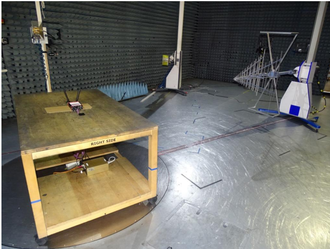
Photo 1: Test setup for radiated measurements (Part 95 - below 1 GHz )
