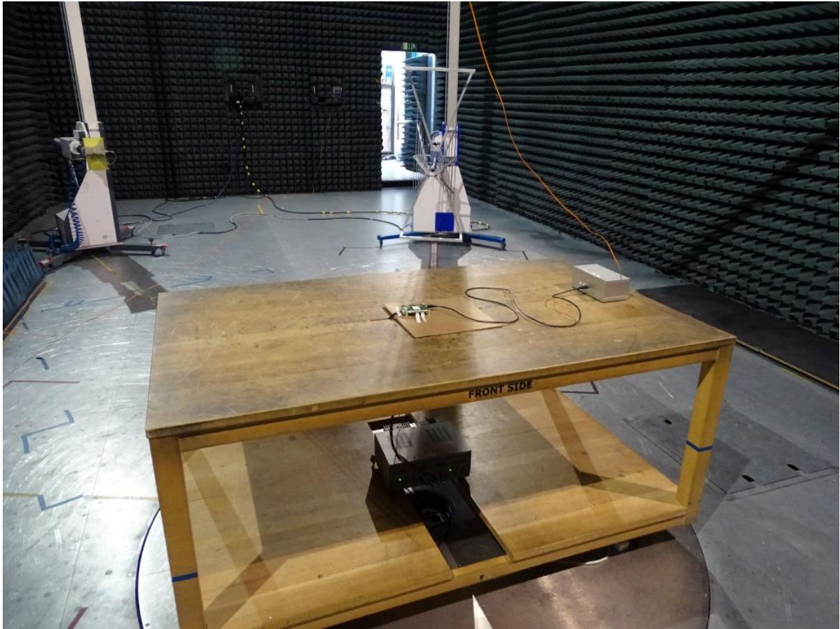
Photo 1: Test setup for radiated measurements (below 1 GHz)
