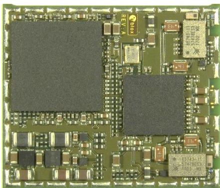
Figure 1: VERA-P173 top view internal photo
