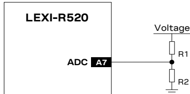
Figure 63: ADC application circuit example
