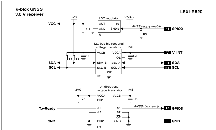
Figure 62: Application circuit for connecting LEXI-R520 modules to a u-blox 3.0 V GNSS receiver
