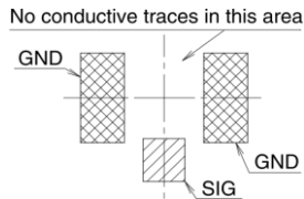
Figure 32: U.FL surface mounted connector mounting pattern layout
