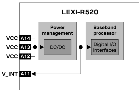
Figure 7: LEXI-R520 interfaces supply output (V_INT) simplified block diagram
