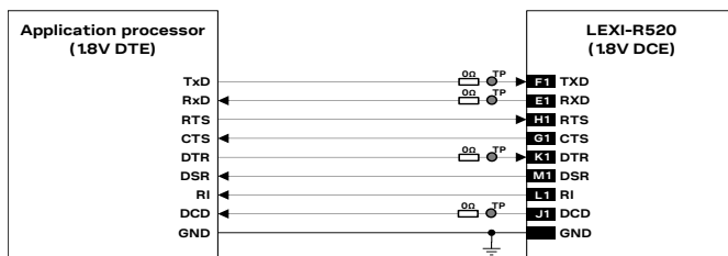
Figure 48: 1 UART interface application circuit with complete V.24 link in DTE/DCE serial communication (1.8 V DTE)
