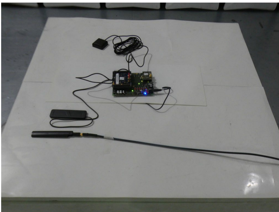
Photo 5: EUT setup for radiated measurements below 1GHz
