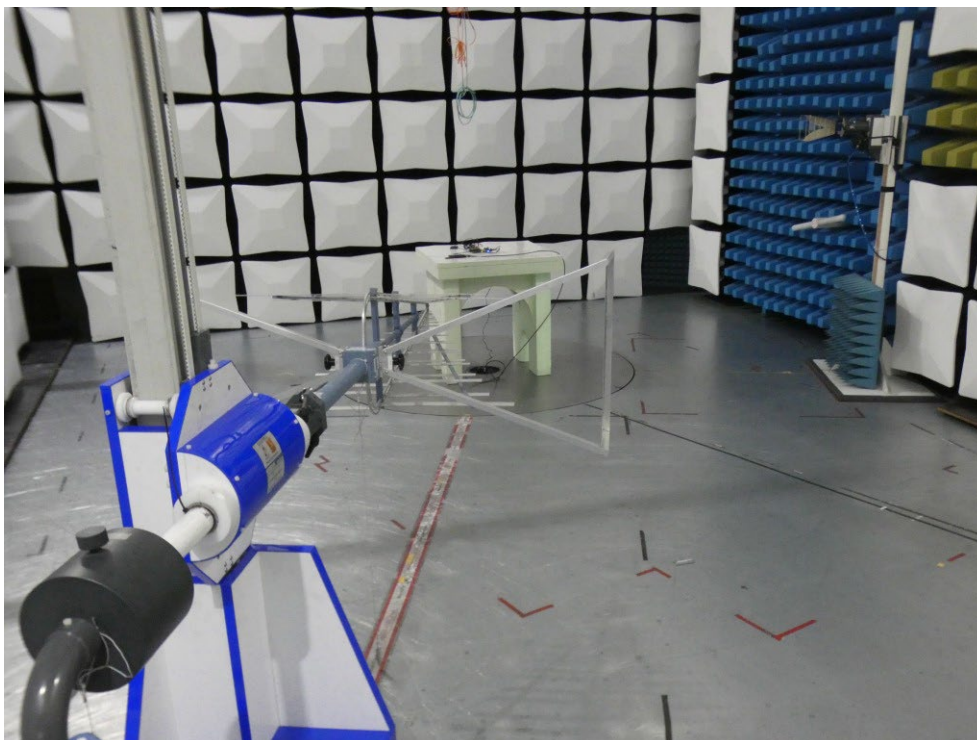
Photo 4: Test setup for radiated measurements below 1GHz
