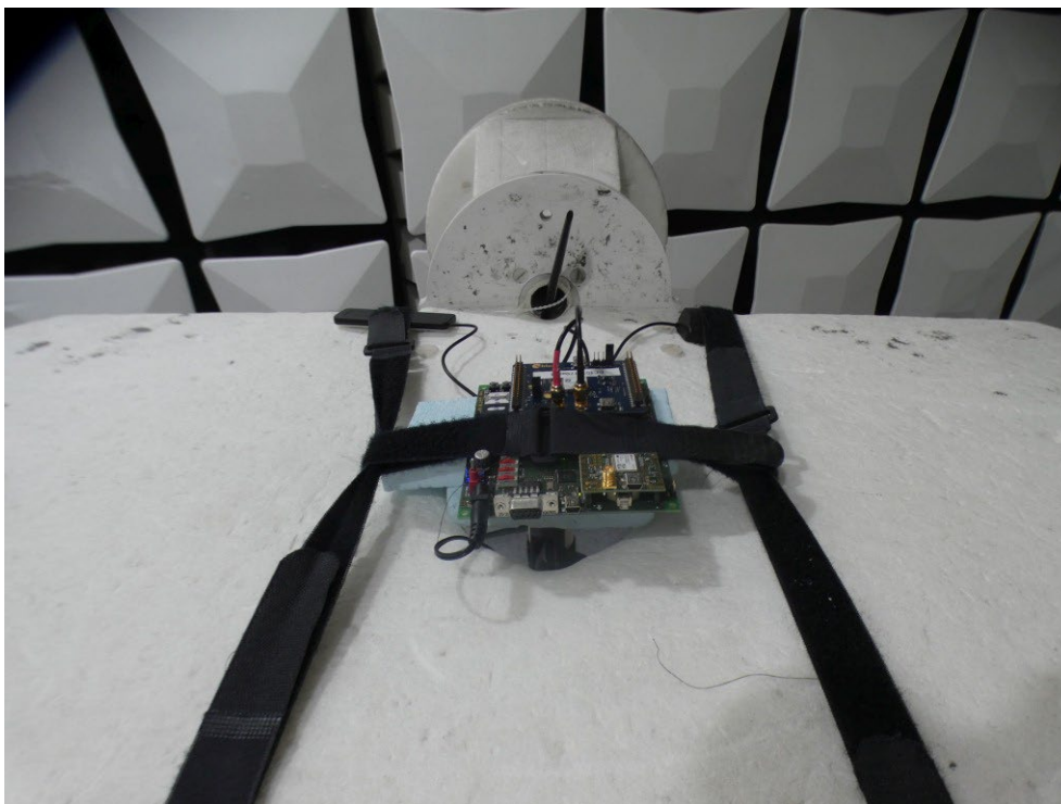
Photo 2: EUT setup for radiated measurements above 1GHz
