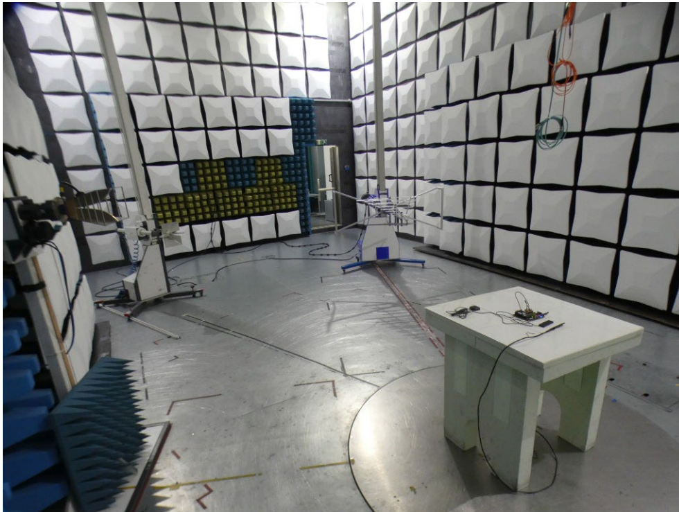
Photo 6: Test Antenna for radiated measurements below 1GHz
