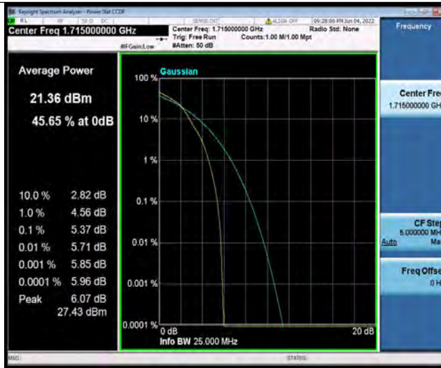
Band4-10MHz-16QAM-20000-27RB#0
