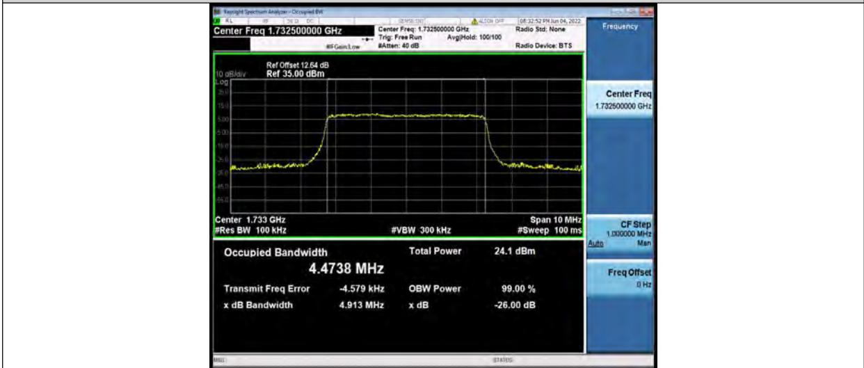
Band4-5MHz-QPSK-20375-25RB#0
