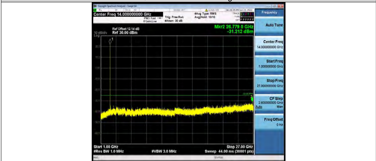
Band41-10MHz-16QAM-39700-1RB#0-Range2:1000~27000MHz
