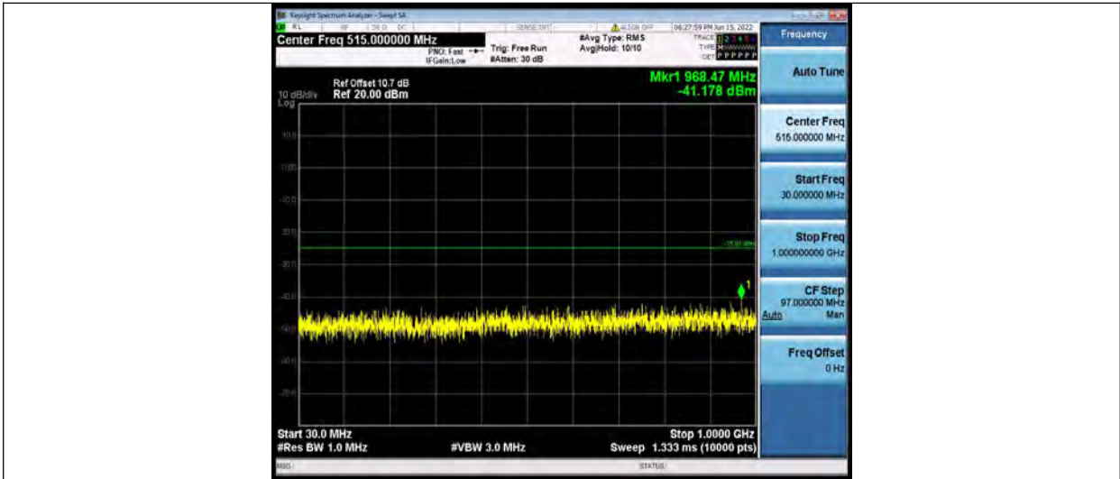
Band41-10MHz-16QAM-40620-1RB#0-Range1:30~1000MHz
