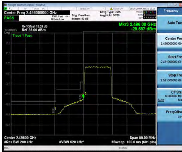
Band41-10MHz-QPSK-41540-1RB#49
