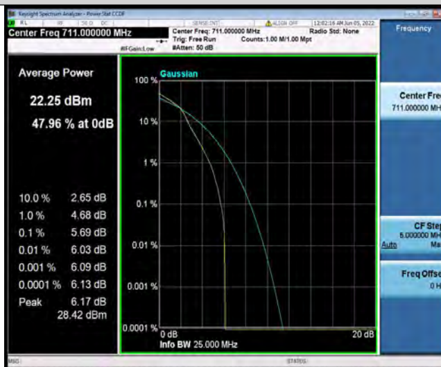
Band12-10MHz-16QAM-23130-27RB#0
