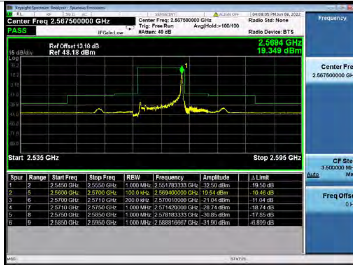
Band7-10MHz-QPSK-21400-50RB#0
