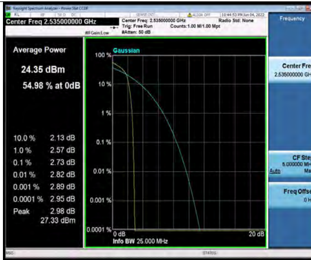
Band7-10MHz-16QAM-21100-27RB#0
