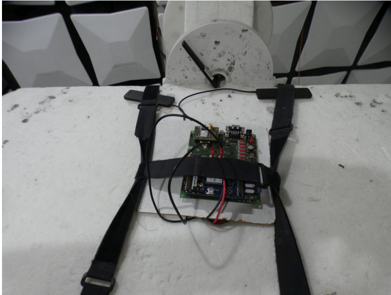
Photo 2: EUT setup
