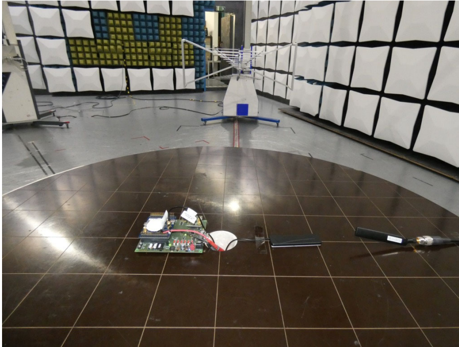
Photo 6: Test Antenna
