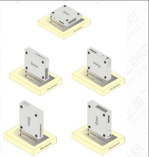
Figure 8.3-1 Test positions for desktop devices
