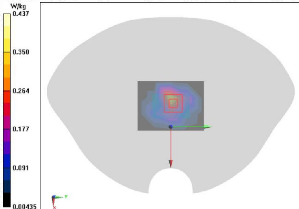
Figure A.1-6 LTE Cat-M Band 66 10MHz 1RB Ooffset Front Side Mode High 0mm
