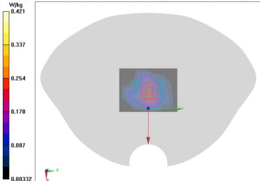
Figure A.1-2 LTE Cat-M Band 4 15MHz 1RB Offset Front Side Mode Low 0mm
