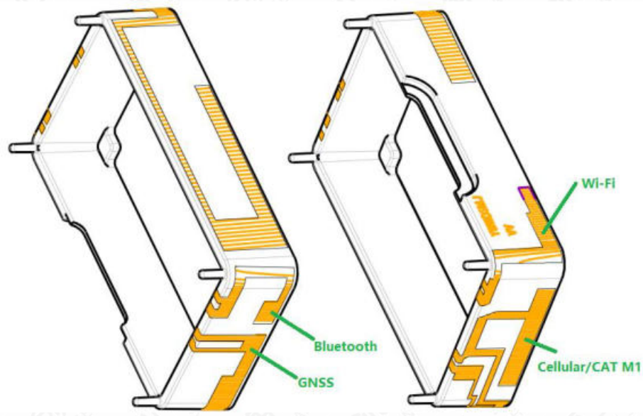
Figure 12.2-3 Antenna Locations
