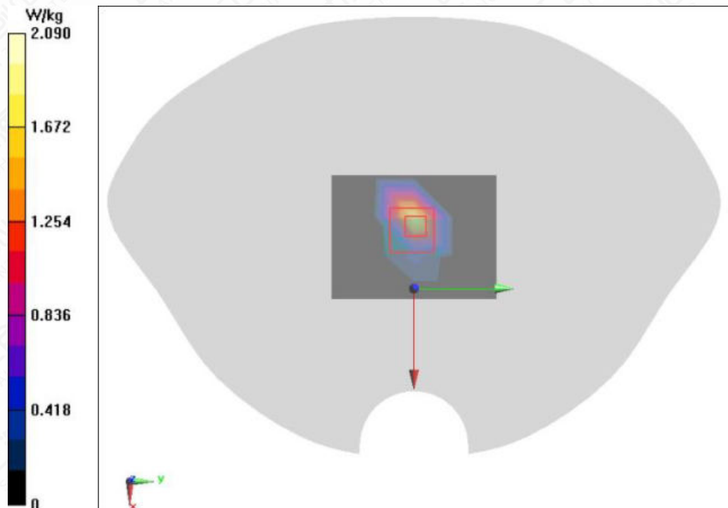
Figure A.1-1 LTE Cat-M Band 2 3MHz 1RB Offset Left Side Mode High 0mm
