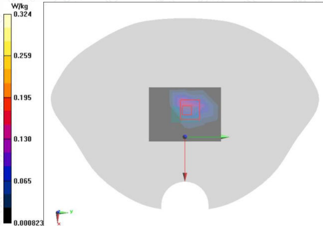
Figure A.1-5 LTE Cat-M Band 13 10MHz 3RB Ooffset Left Side Mode Middle 0mm
