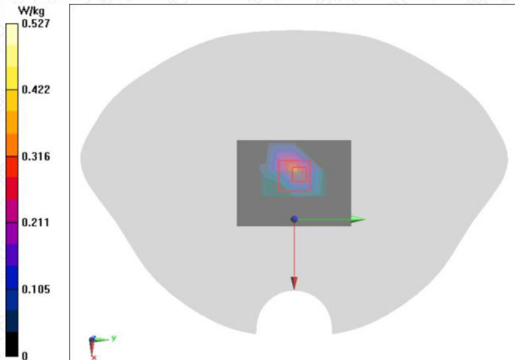
Figure A.1-4 LTE Cat-M Band 12 10MHz 3RB Ooffset Top Side Mode Middle 0mm
