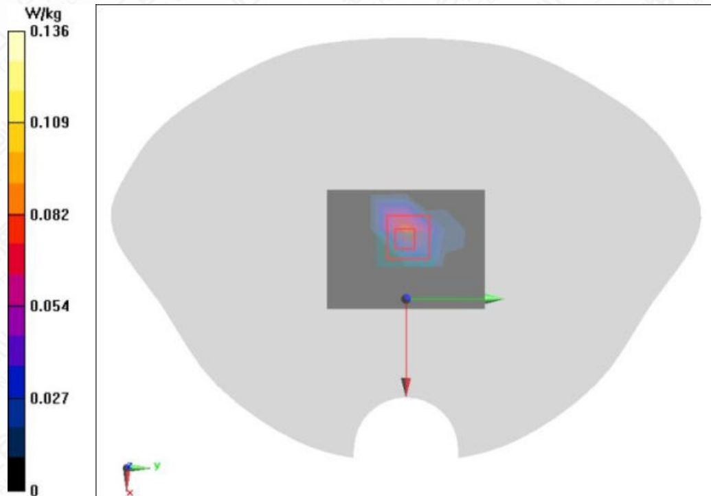
Figure A.1-3 LTE Cat-M Band 5 10MHz 1RB Offset Left Side Mode Middle 0mm
