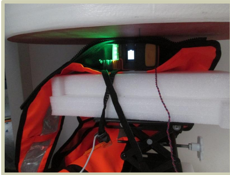
WI-FI TESTING SIM CARD SIDE
