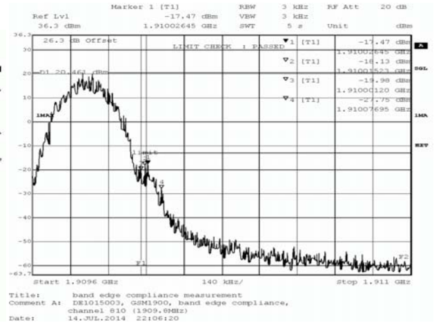
GSM 1900 Band
