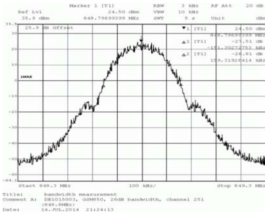
GSM 850 Band
