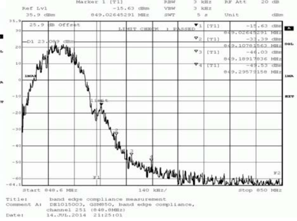
GSM 850 Band
