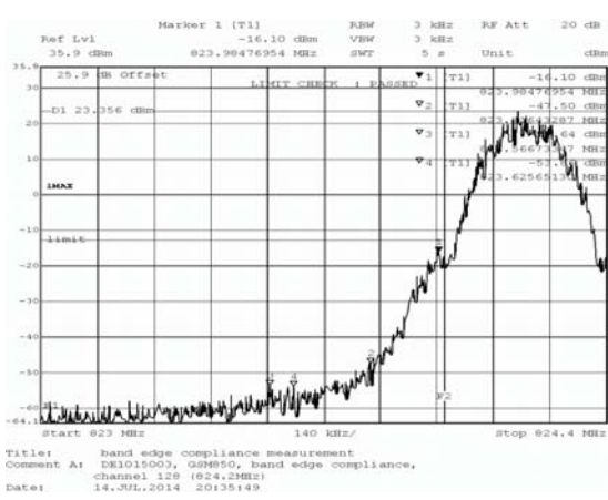
GSM 850 Band
