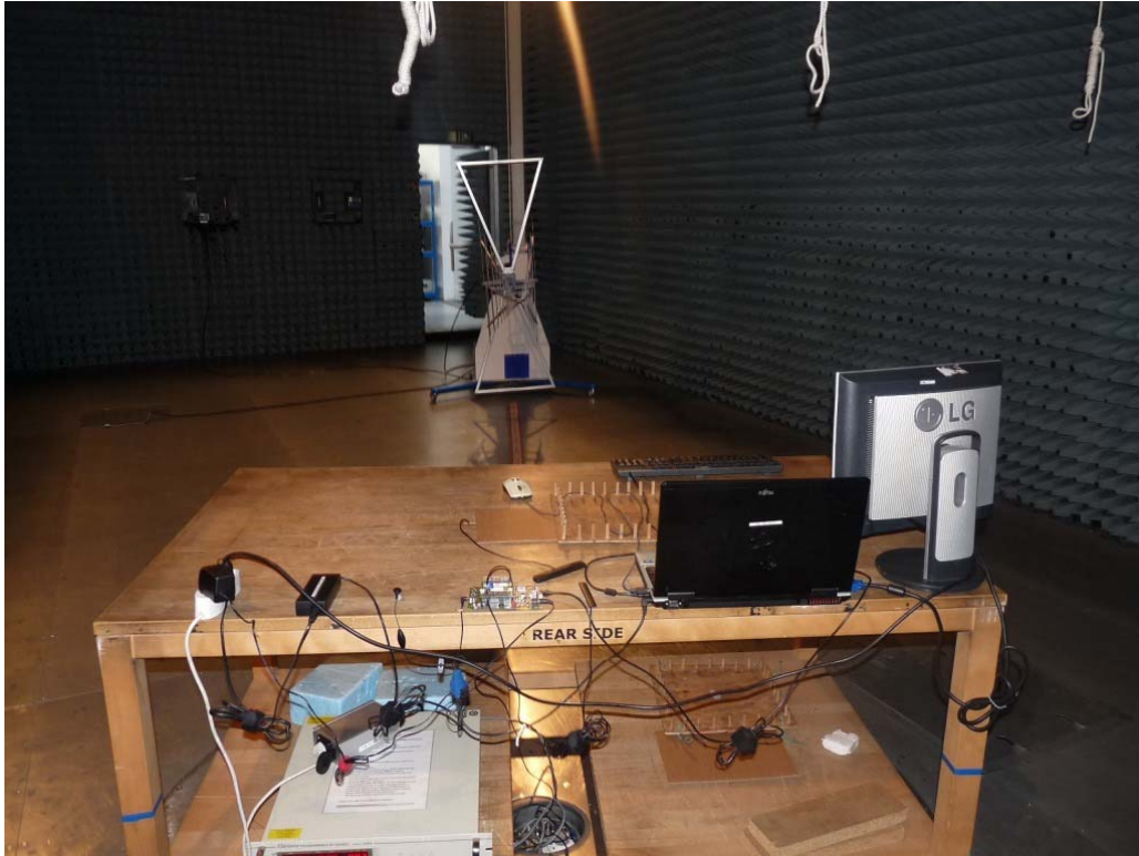
Photo 8: Test setup for radiated measurements (computer peripheral setup, EUT supplied by ACDC Adapter, unintentional radiator S15)
