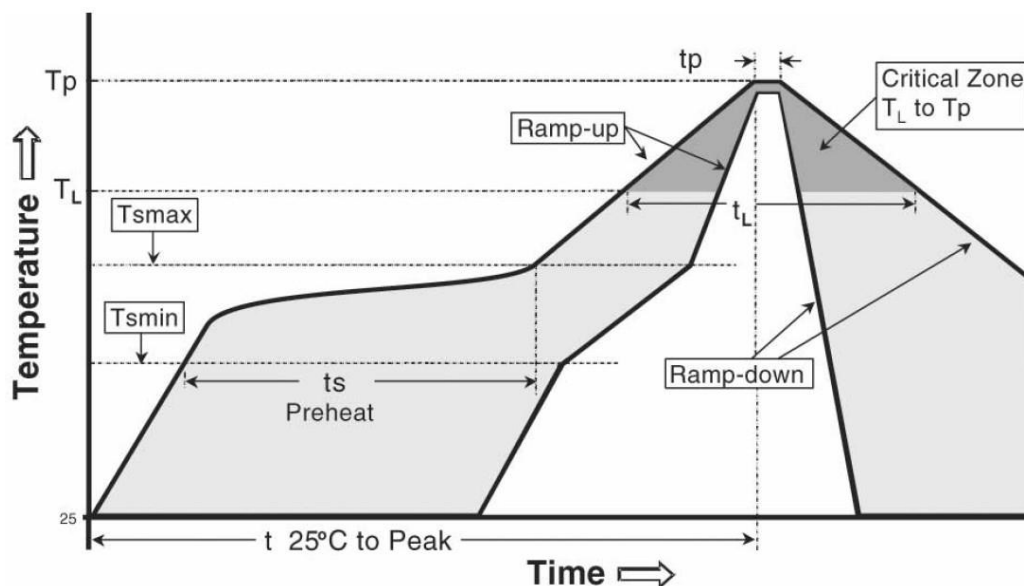
Figure 16: Reflow profile
