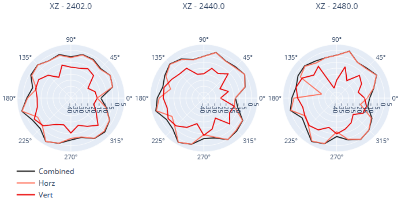
Figure 2 - Gain X-Z
