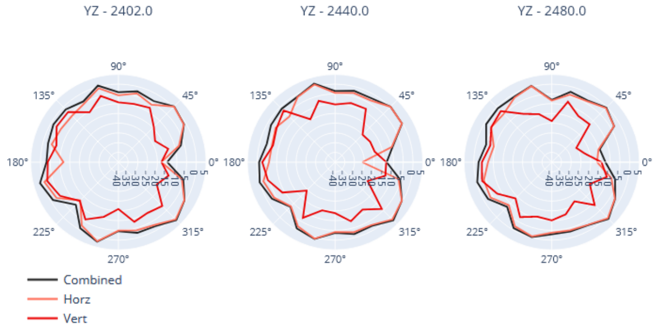
Figure 3 - Gain Y-Z
