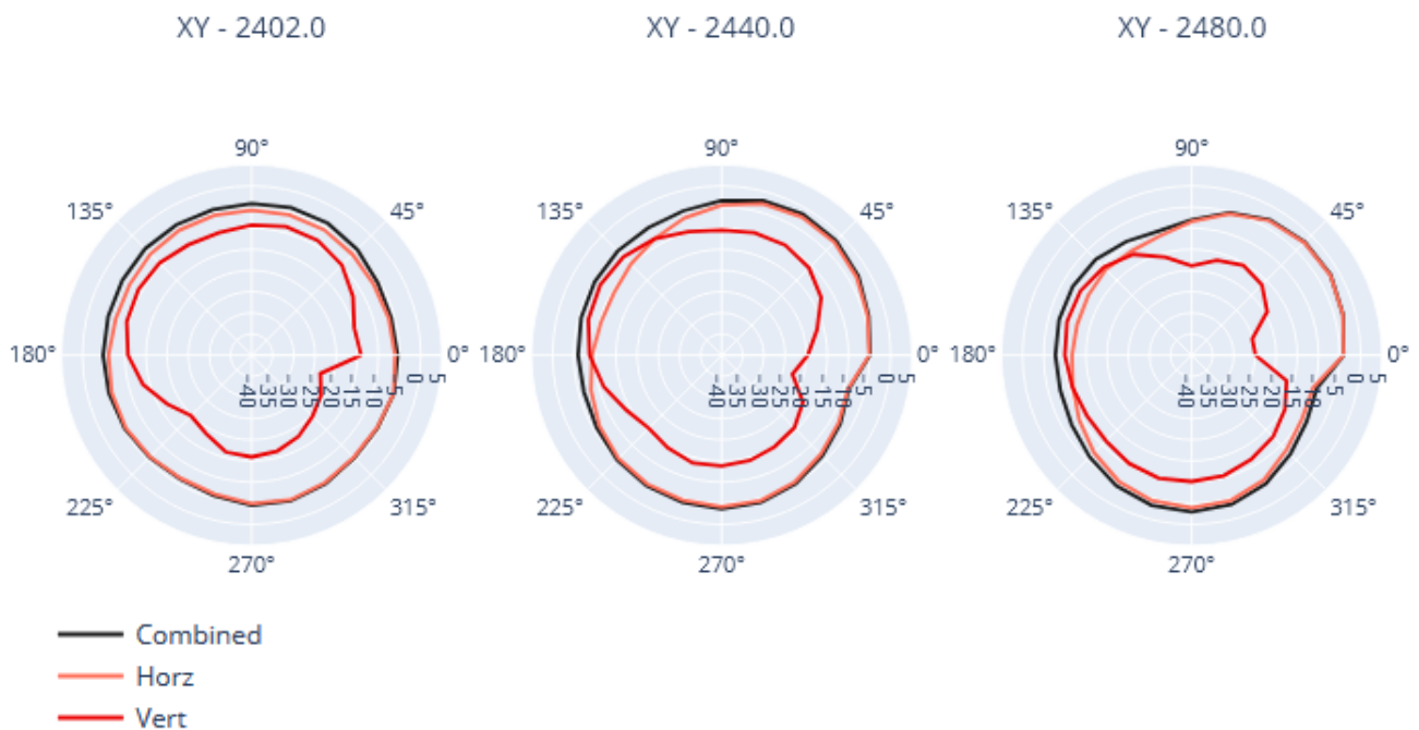
Figure 1 – Gain X-Y
