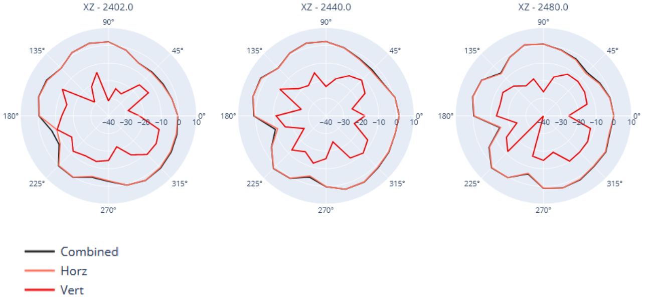
Figure 2 - Gain X-Z
