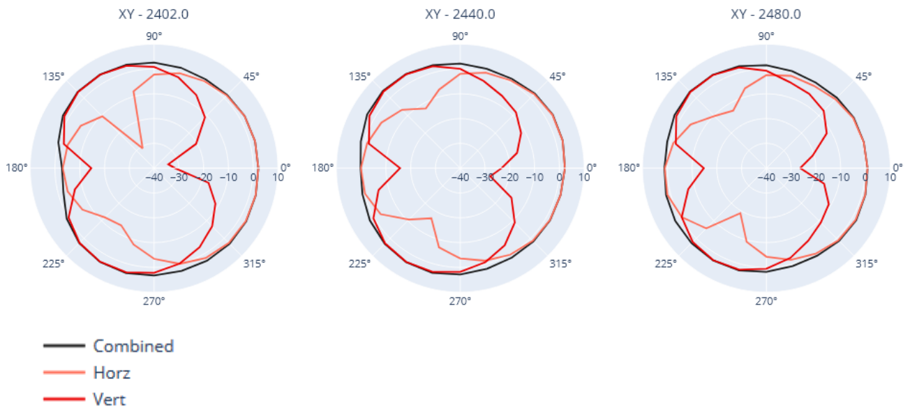
Figure 1 – Gain X-Y
