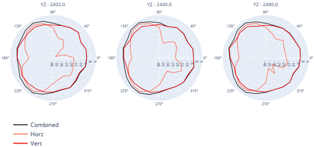
Figure 3 - Gain Y-Z
