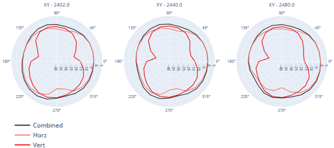
Figure 1 – Gain X-Y
