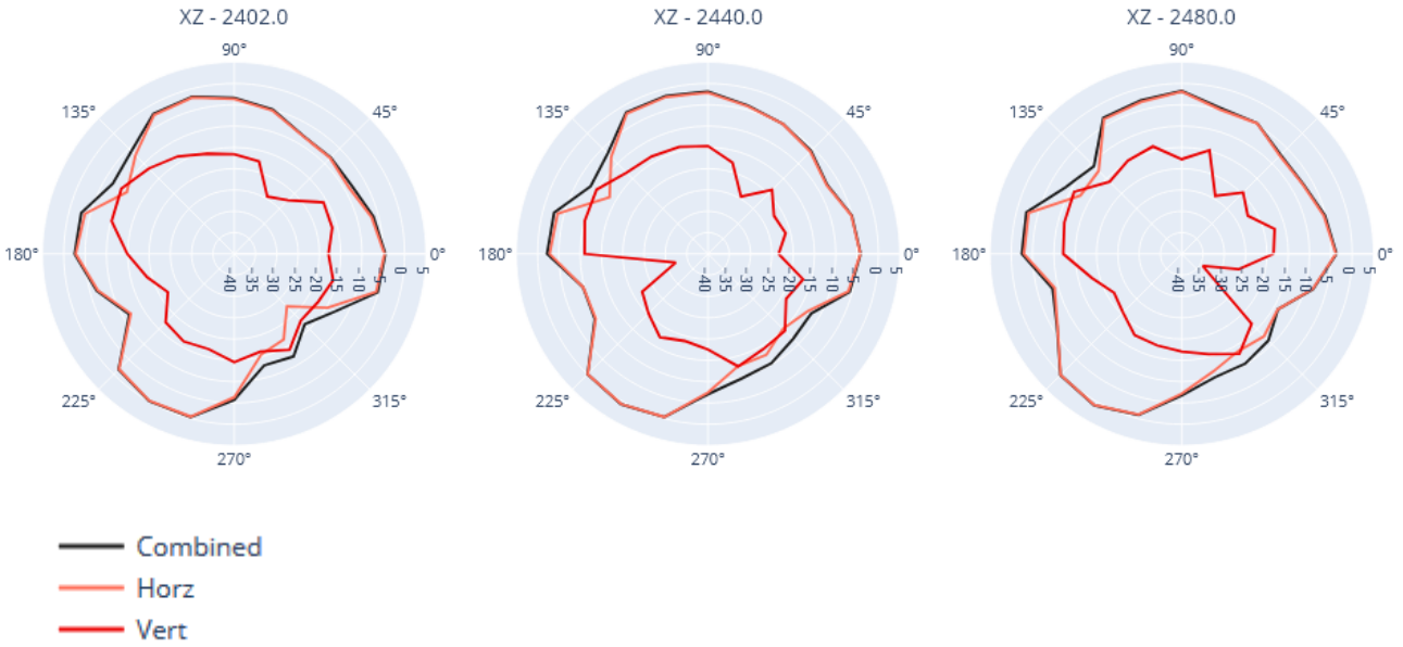
Figure 2 - Gain X-Z
