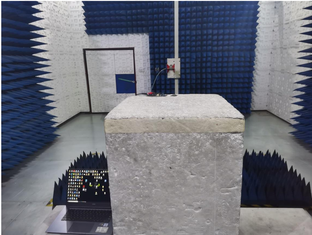
RADIATED EMISSION TEST SETUP ABOVE 1GHZ-NORA-B106
