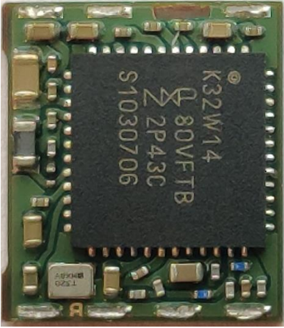
Figure 3: NINA-B501 external photo
