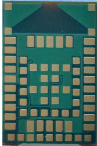
Figure 6: NINA-B506 external photo
