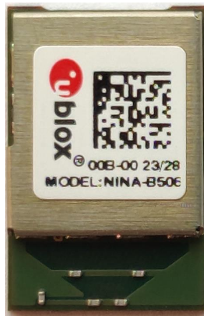
Figure 2: NINA-B506 external photo
