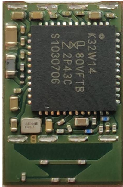
Figure 4: NINA-B506 external photo
