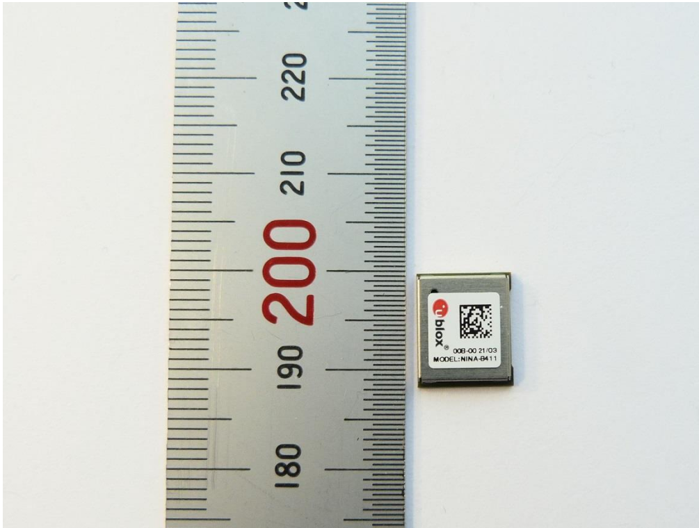
TOP VIEW OF EUT (NINA-B411)
