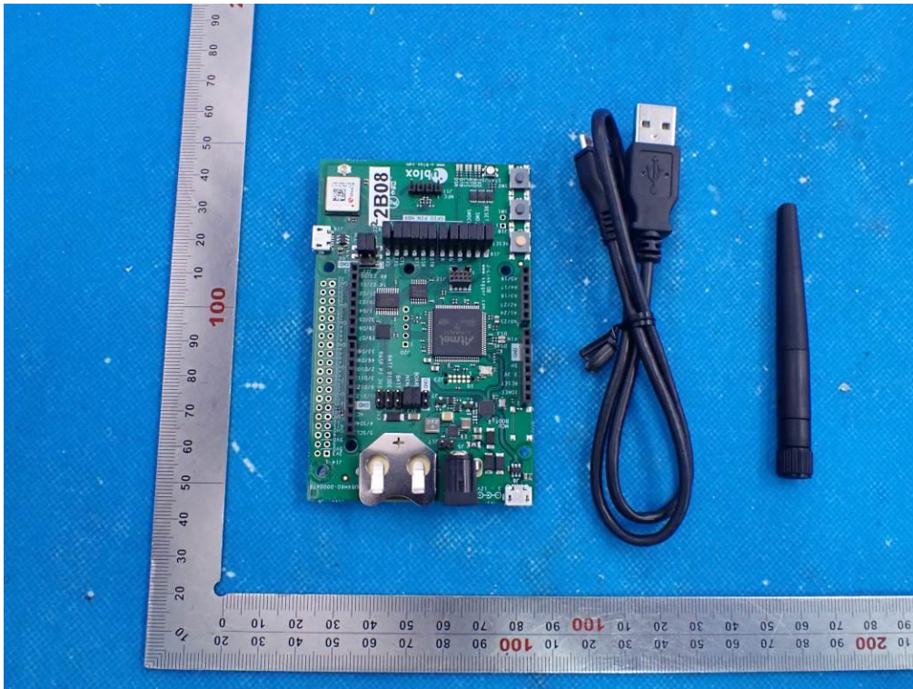
ALL VIEW-1 OF EUT (NINA-B411)
