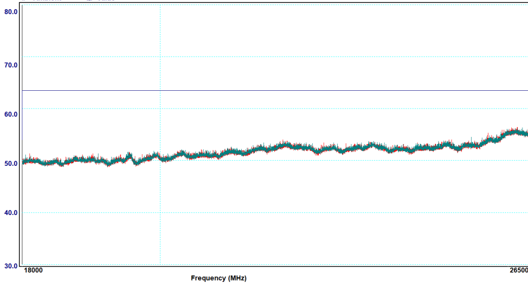
Graph 6-17: Transmitter Spurious Emissions, 18– 26 GHz, 2440 MHz, Average
