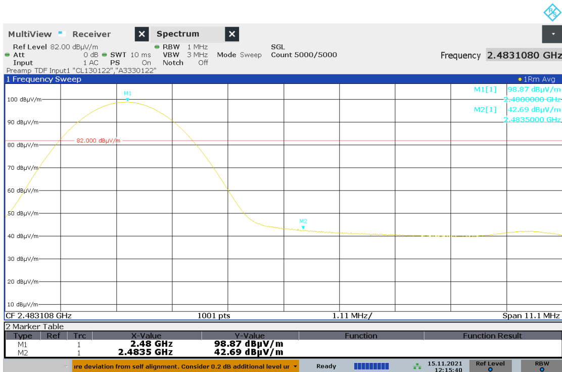
Graph 6-21: Upper Band-edge, Average
