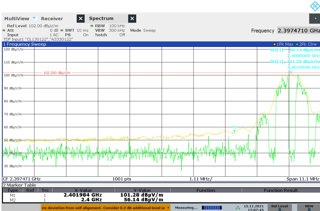
Graph 6-19: Lower Band-edge
