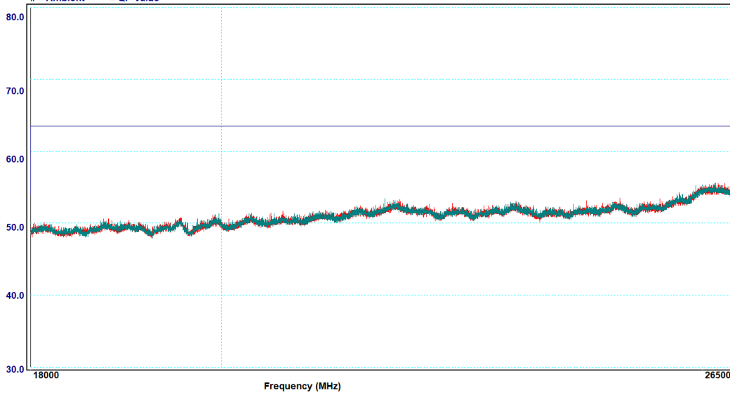
Graph 6-16: Transmitter Spurious Emissions, 18– 26 GHz, 2402 MHz, Average
