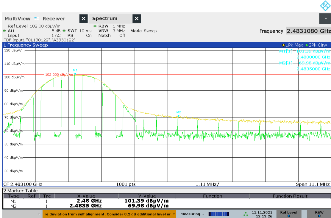
Graph 6-20: Upper Band-edge, Peak
