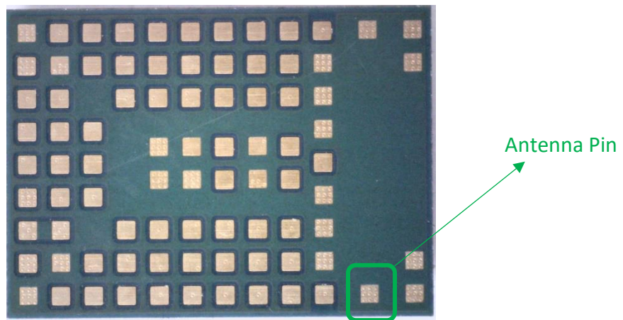
Figure 3: Bottom view of MAYA-W276-00B and MAYA-W266-00B
