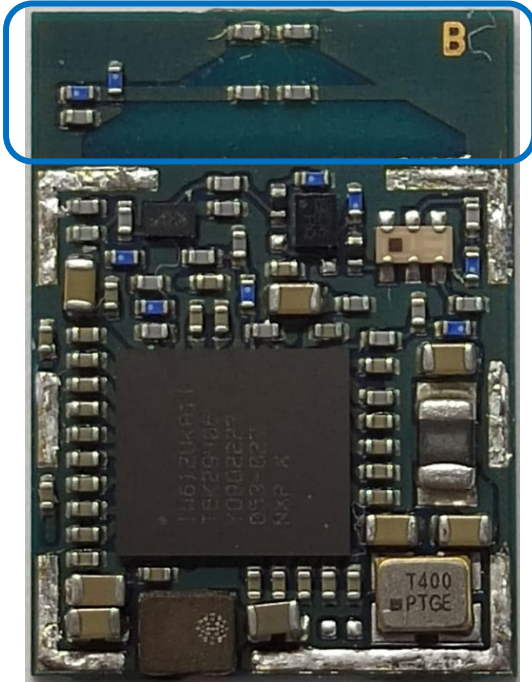
Figure 4: MAYA-W276-00B top view internal photo
