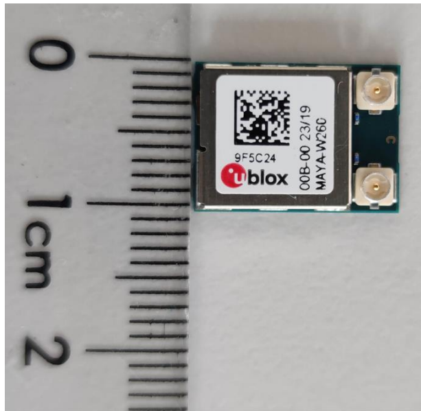
Figure 6 MAYA-W260-00B external photo 2
