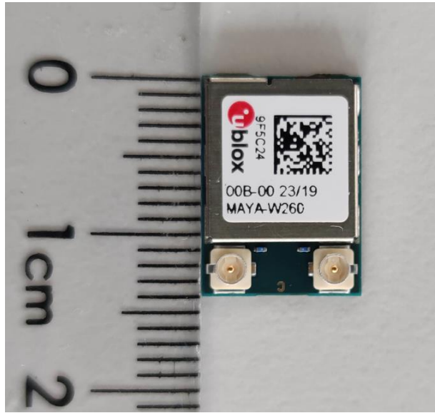
Figure 5 MAYA-W260-00B external photo 1
