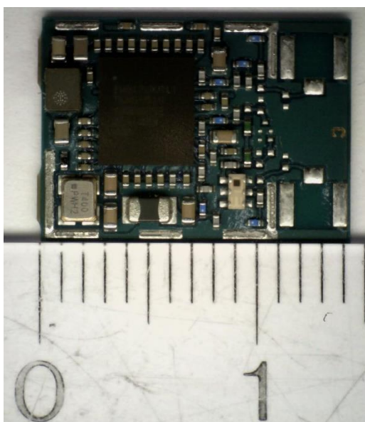
Figure 8 : MAYA-W261-00B top view length
