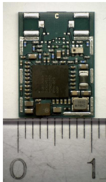
Figure 11 : MAYA-W271-00B top view width
