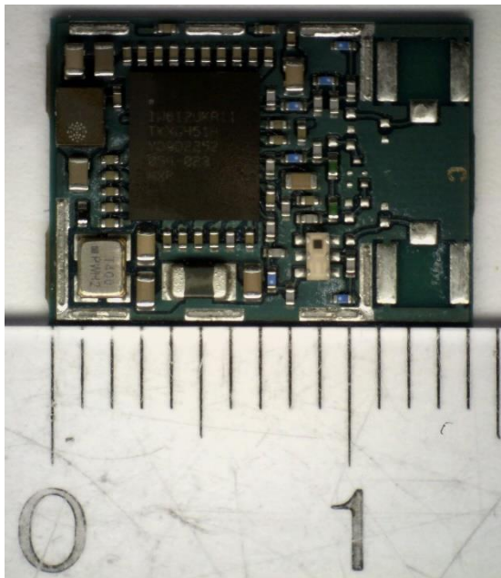
Figure 10 : MAYA-W271-00B top view length
