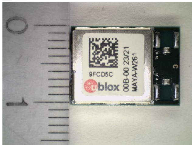
Figure 2 MAYA-W261-00B external photo 2
