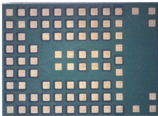
Figure 7: Bottom view of MAYA-W271-00B, MAYA-W261-00B and MAYA-W260-00B
