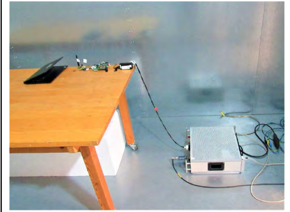
Setup for measurements 150 KHz - 30 MHz
