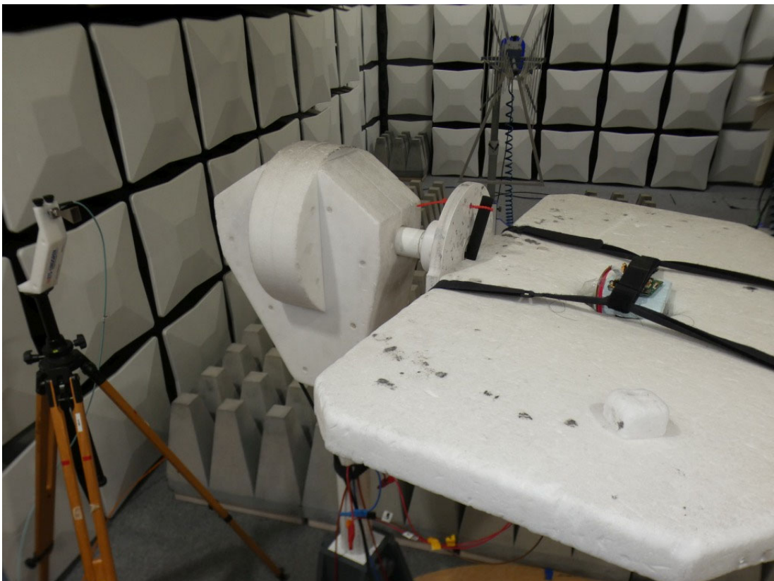
Photo 4: Test setup for radiated measurements above 26 GHz
