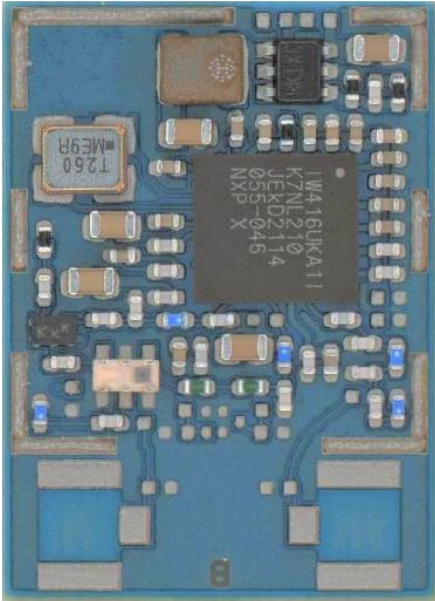
Figure 3: MAYA-W161-00B module internal photo
