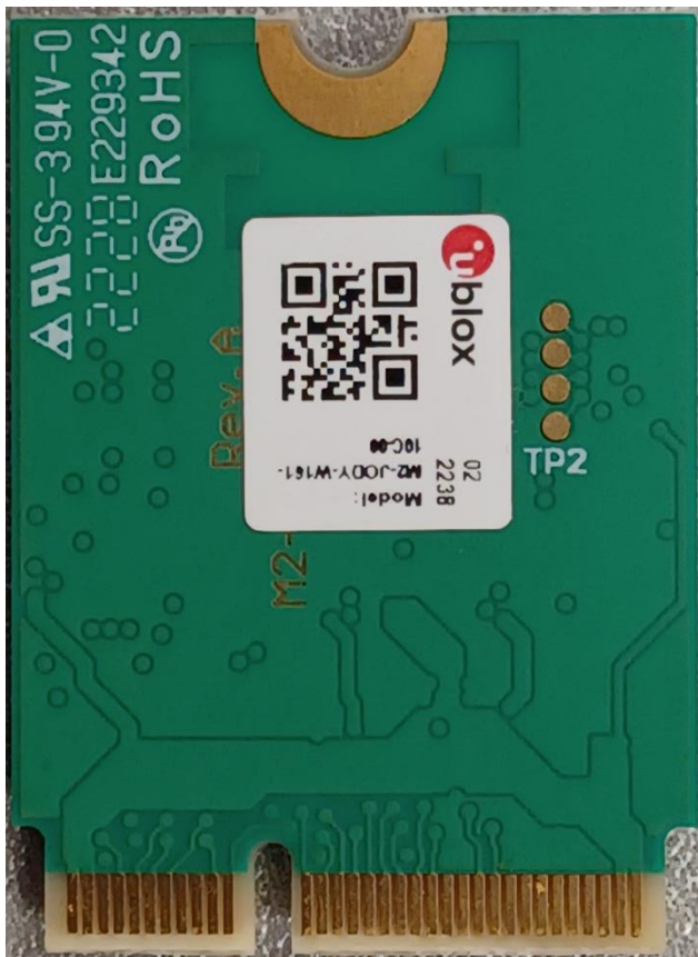
Figure 1: M2-MAYA-W161 bottom view external photo
