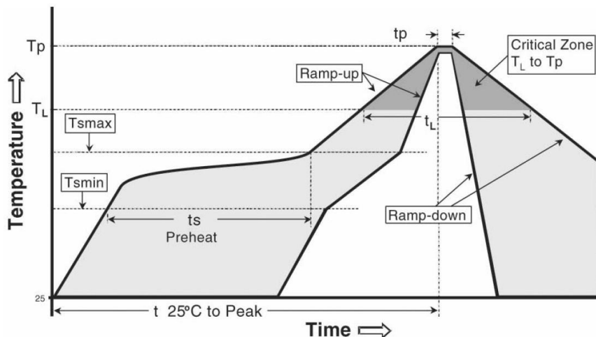
Figure 17: Reflow profile
