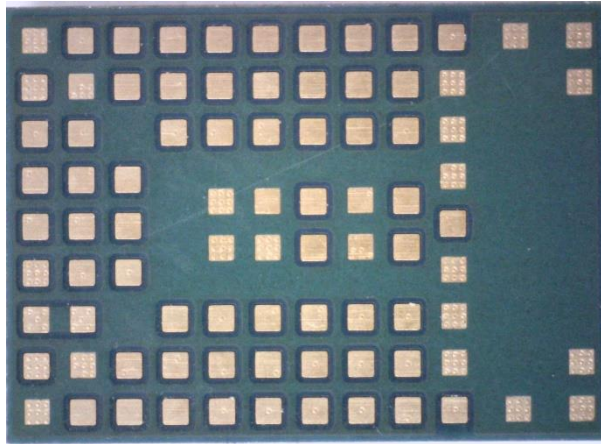
Figure 9: Bottom view of MAYA-W160-00B, MAYA-W161-00B, MAYA-W166-00B and MAYA-W166-01B
