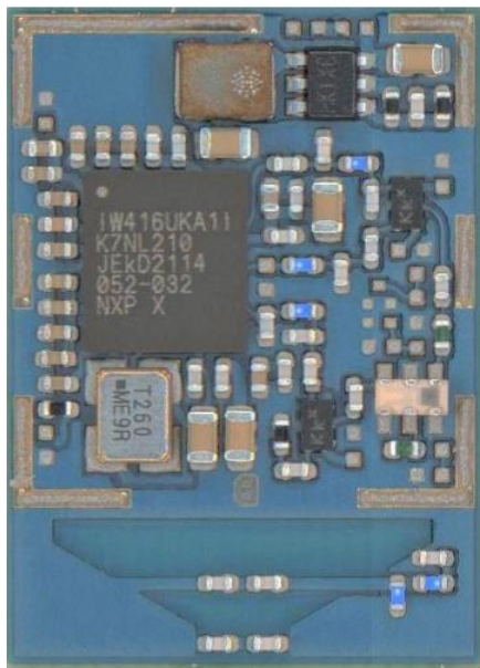
Figure 3: MAYA-W166-00B internal photo
