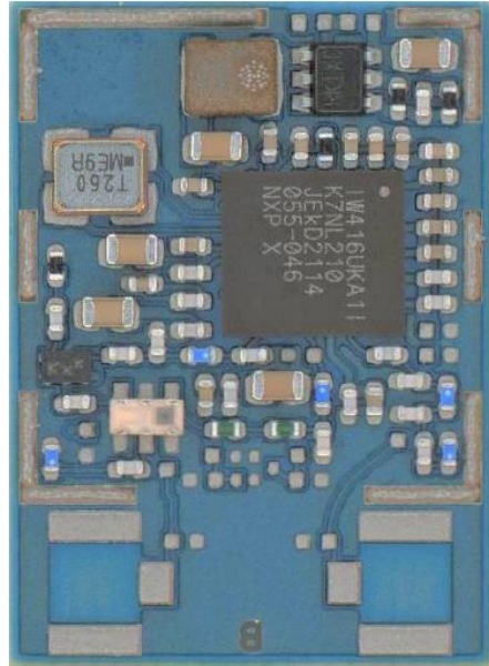
Figure 2: MAYA-W161-00B internal photo
