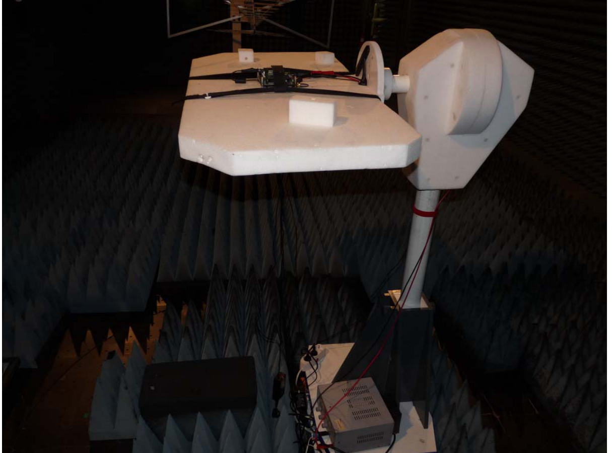
setup for the test spurious emissions radiated
