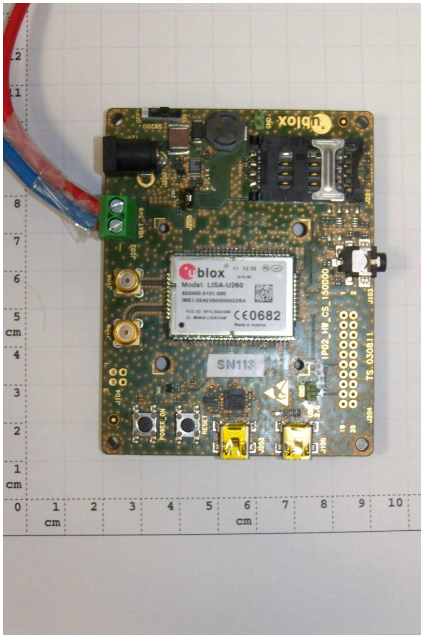
EUT A top view (RF Data-module plug on the middle of EUT B (Adapter board))
