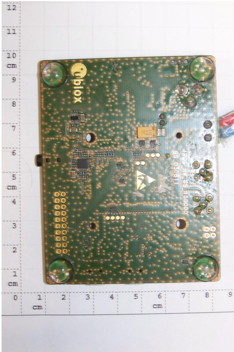
EUT A bottom view
